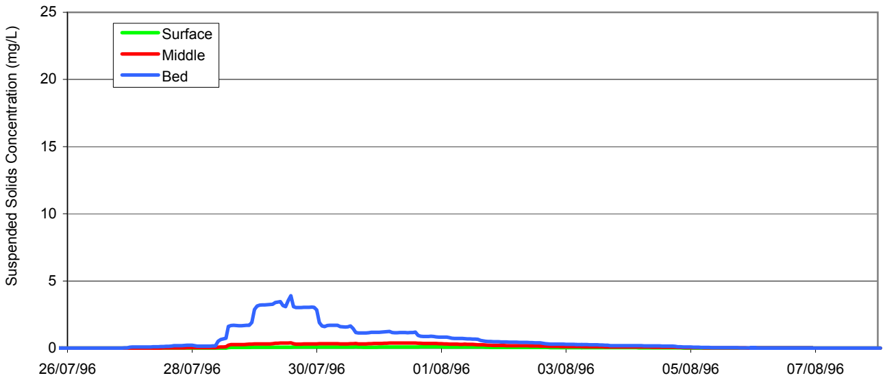
Figure 6.11 Daily Averaged Suspended Solids Concentration, East of Sha Chau
