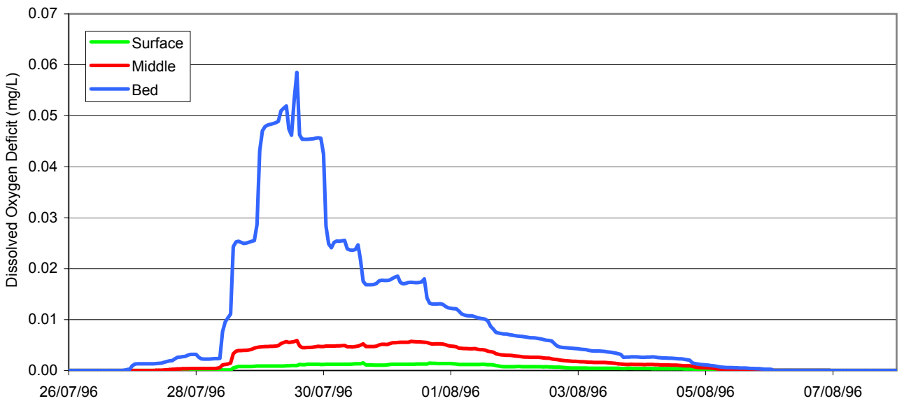
Figure 6.12 Daily Averaged DO Deficit (mg/L) at East of Sha Chau
